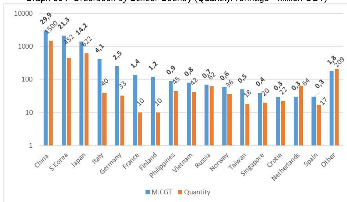
Graph 39 : Orderbook by Builder Country (Quantity/Tonnage - Million CGT)
